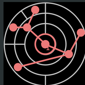
(b) Sunburst
