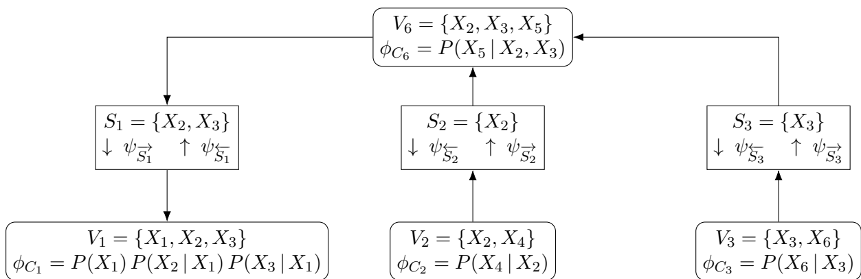
Figure 5.3: Illustration of the message boxes and potentials used for message passing in junction trees, based on the junction tree shown in Figure 5.2. For this tree, V_1 is chosen as the root node. The arrow directions depict the forward pass, the backward pass goes in reverse.
