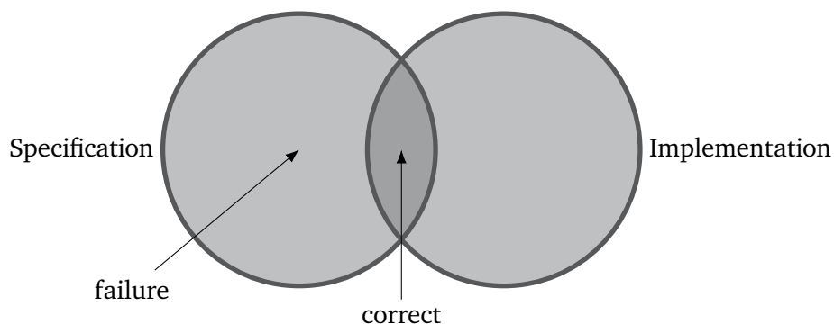
Figure 6.1: Taxonomy of Software Misbehavior
