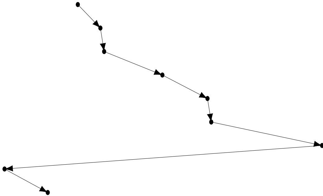
Figure 9.9: FS Scheduling: C-LOOK
